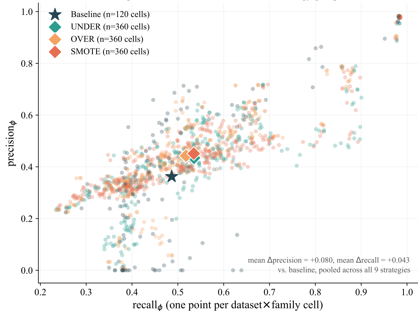
Precision-recall plane, all 1200 raw cells (faded) with strategy-group means (solid)
